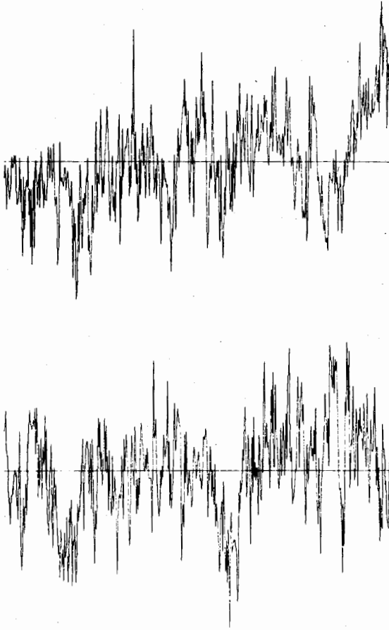
FIGURE 11 (top) 1/f noise produced by filtering a sample of Gaussian white noise. The impulse response of the filter is G_-(t - t_0) of Eq. (2), the fully retarded (causal) response. (bottom) Same as top figure, except the response is here G_+(t - t_0) , the fully advanced (acausal) response. Figure 4 also shows filtered white noise; its response function is 1/2 (G_+ + G_-) .
